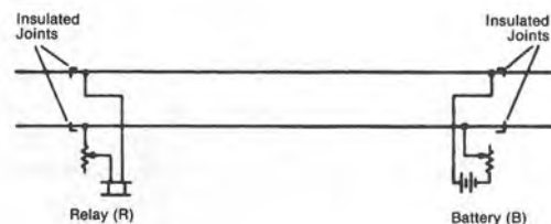
Figure 41. DC Track Circuit
