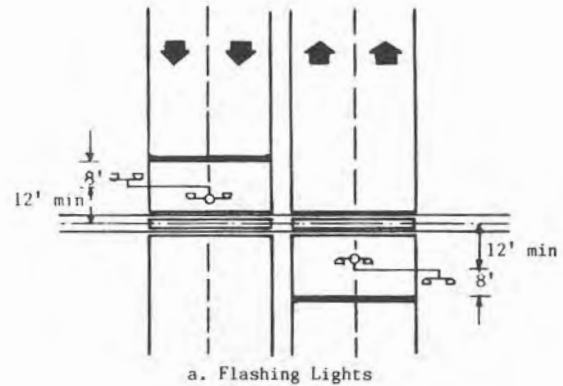
Figure 34. Typical Location Plan, Divided Highway with Insufficient Median for Signals, Two Lanes Each Way
